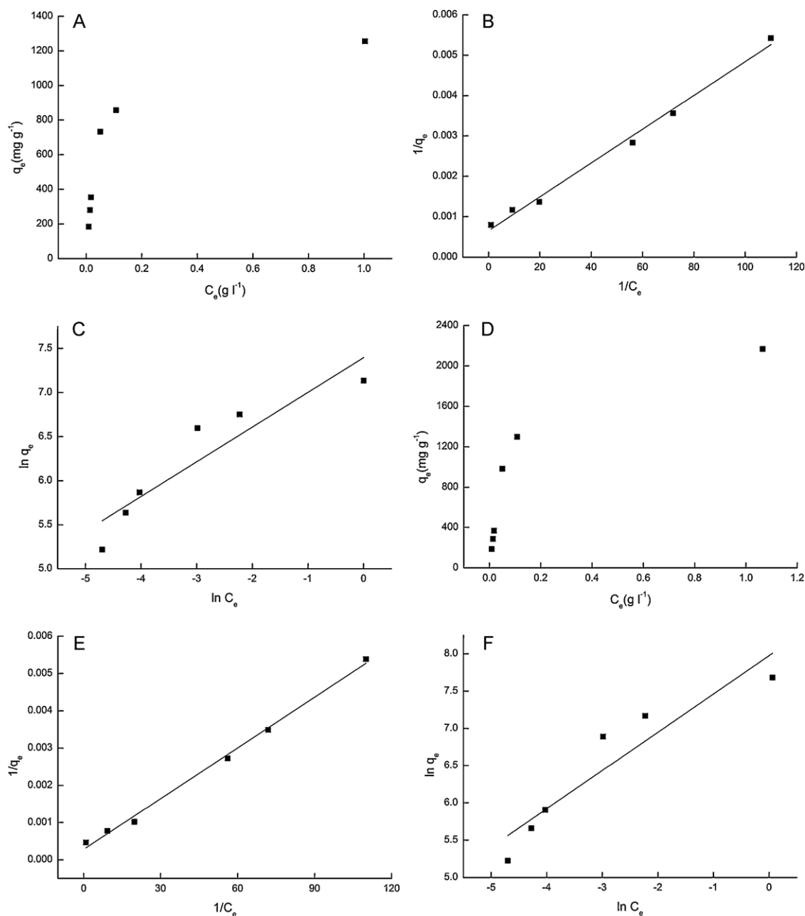
Fig. 9. Adsorption isotherms of GO (A) and SRGO (D), and their results fitted by the Langmuir model (B and E) and the Freundlich model (C and F).
