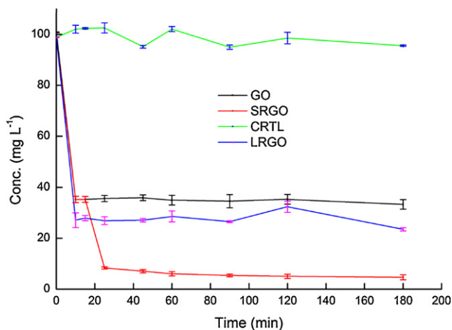
Fig. 7. Time-dependent adsorption of AO (100 mg L ^{-1} ) with GO, SRGO, and LRGO (additive amount of GO: 1 mL) compared to AO in reducing solution (CTRL), at room temperature. Note: for SRGO, adsorption was performed with addition of the reductant at the 15th minute (removal efficiency about 95%); for LRGO, GO was pre-treated with reductant overnight at room temperature with removal efficiency of 76%; for GO, removal efficiency was about 67%.
