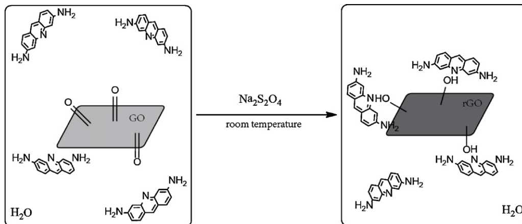
Fig. 15. Possible mechanism for the AO sorption enhancement.
