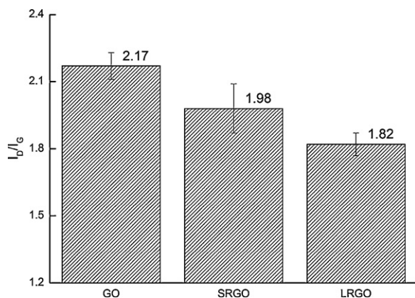
Fig. 11. Histogram of I_D/I_G ratios from Raman spectra of GO, SRGO, and LRGO.
