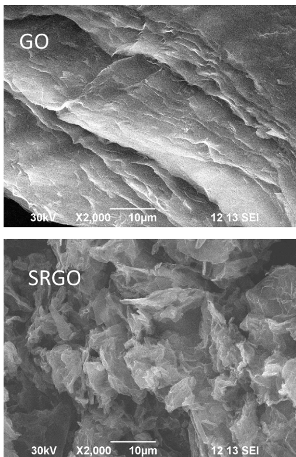
Fig. 10. SEM images of GO (upper) and reduced GO (lower).
