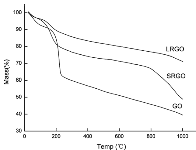
Fig. 14. Thermo-gravimetric analysis for GO, SRGO, and LRGO.
