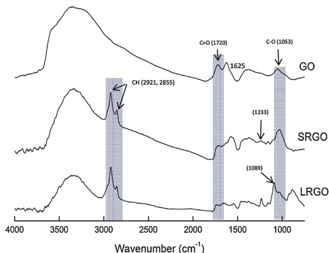
Fig. 13. Fourier transform infrared spectra (vs. absorbance) of as-prepared GO, SRGO, and LRGO.
