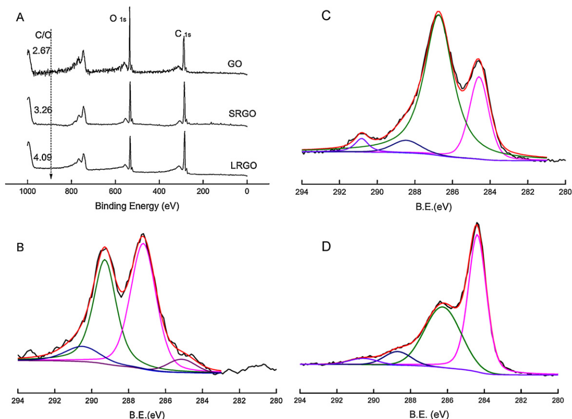
Fig. 12. XPS general spectra and curve fit of C1s spectra of GO, SRGO, and LRGO.
